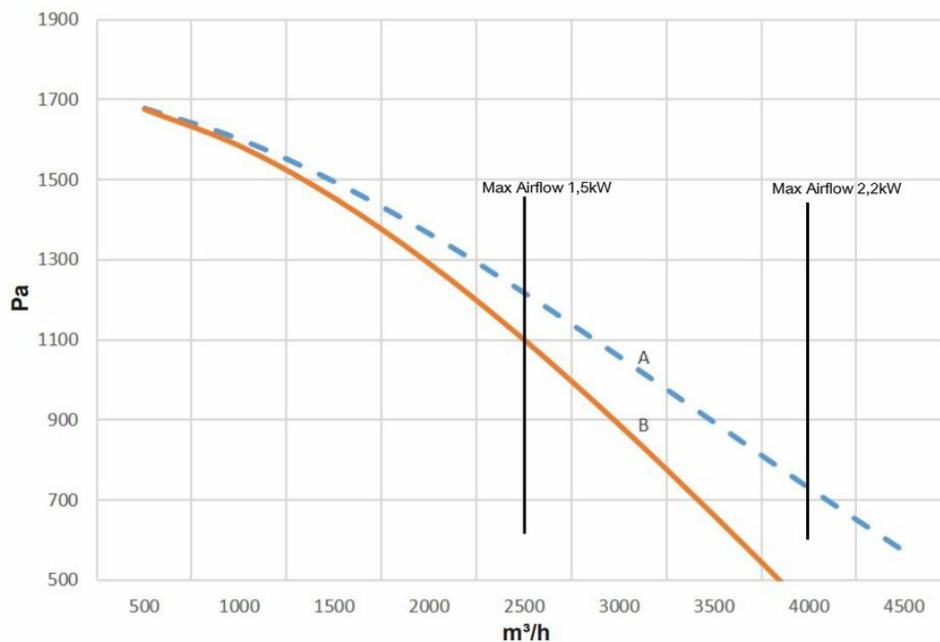
A: Total Pressure B: Static Pressure X: m³/h Y: Pa
